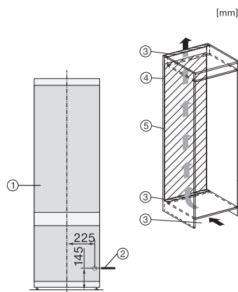
KF7731E, KF7731D, Installation
