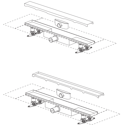
RainDrain Compact 56162800 - 56185000
