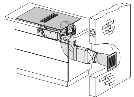
KMDA7676-1FL, KMDA7876-1FL, KMDA7676FL, KMDA7876FL – Einbauvariante 10 Abluft 1) DFK-AK 90, 2) DFK-R 1000, 3) DMK 150-1
