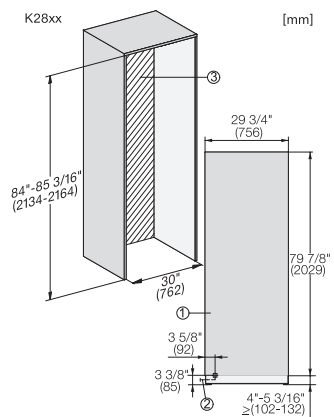
K2801Vi, K2811Vi, K2801SF, K2811SF, Installation, MasterCool, *Fußnote, Skizze
